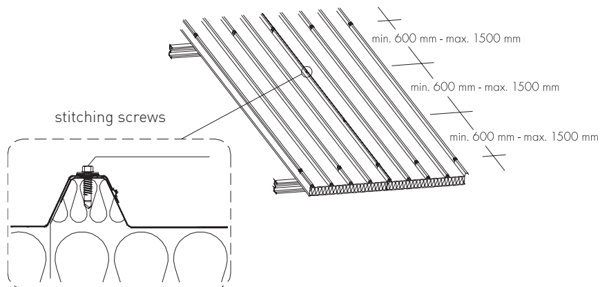
Fig. 21: Stitching screws on a longitudinal joint.
