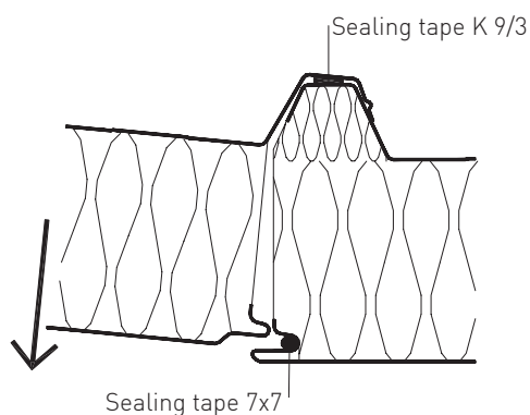
Fig. 20: Panel laying.
