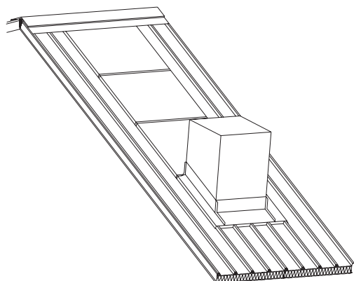
Fig. 24: Installation of an opening on a roof using a steel sheet
