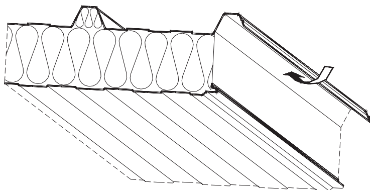
Fig. 15: Checking of trapezoidal panel section.
