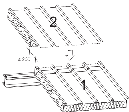
Fig. 22: Sealing of panel extension.
