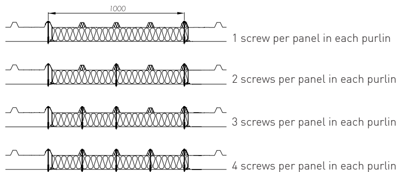
Fig. 1: Fixing arrangement.
