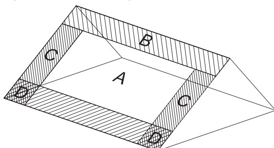
Fig. 2: Characteristic fixing areas.
