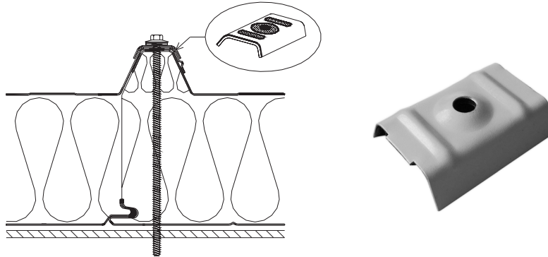
Fig. 26: Fixing method of Trimoterm SNV roof panels.
